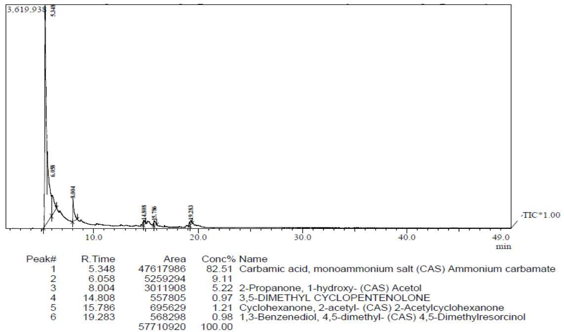
Gambar 6. Kromatogram impregnan dari ekstrak kulit batang sawit Figure 6. Chromatogram of the impregnant made from oilpalm-bark extract
