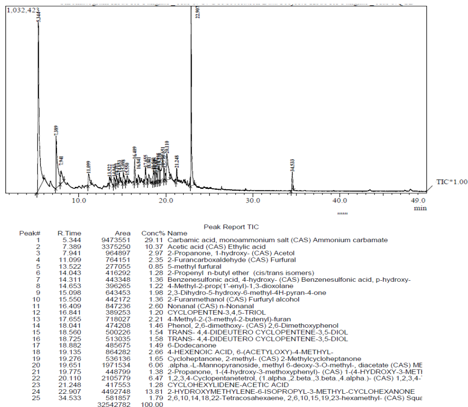
Gambar 2. Kromatogram Py-GCMS ekstrak kulit batang sawit Figure 2. Py-GCMS chromatogram of oilpalm-bark extract
