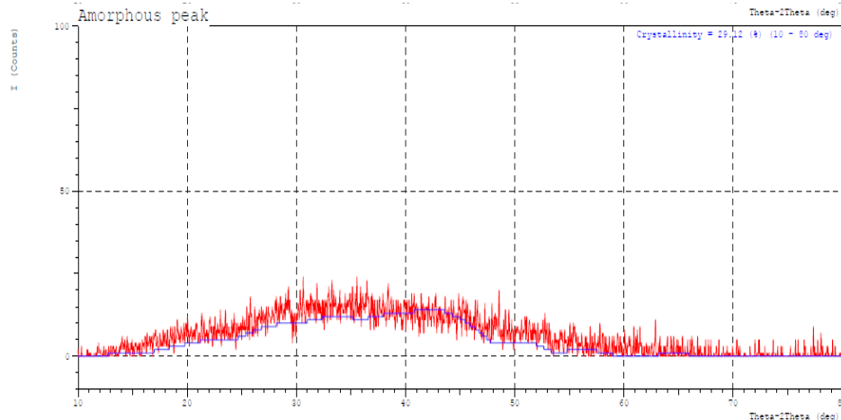
Gambar 7. Difraktogram impregnan dari ekstrak kulit batang sawit Figure 7. Difractogram of the impregnant made from oilpalm-bark extract
